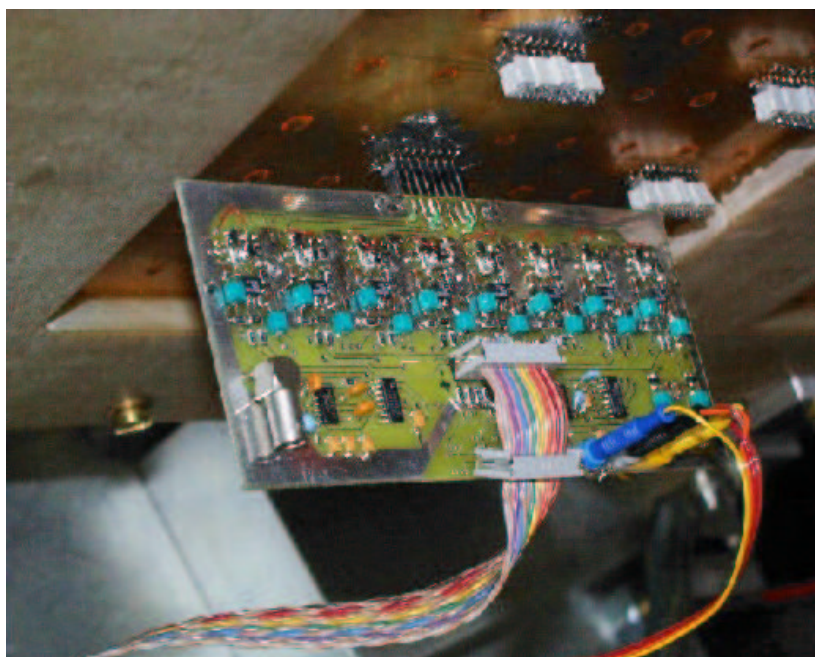
current sensitive PA
