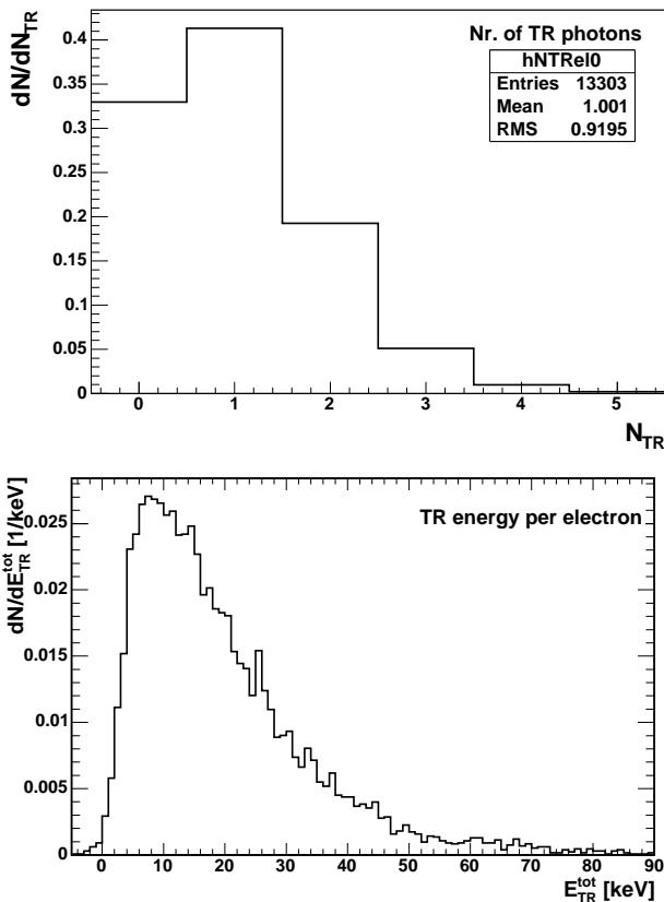
Figure 1: Top panel: Distribution of the number of photons detected in the drift chamber at a momentum of 8 GeV/c. Bottom panel: Spectrum of energy deposited in the detector by TR.
