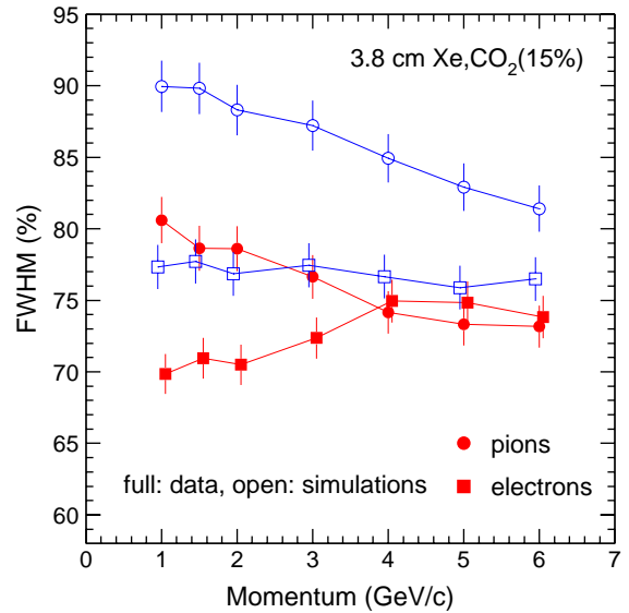
Fig. 8. Momentum dependence of the FWHM value of the energy loss normalized to MPV for pions and electrons. Full symbols are measurements, open symbols are calculations.
