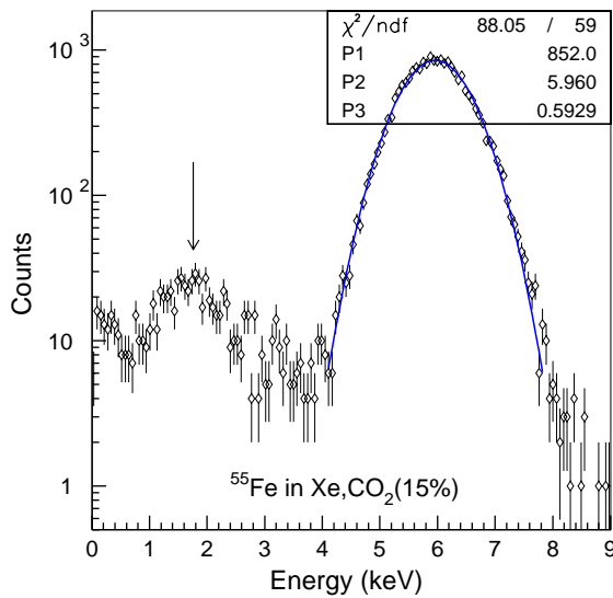
Fig. 1. ^{55}\text{Fe} spectrum in \text{Xe}, \text{CO}_2(15\%) . A Gaussian fit of the main peak of 5.96 keV is also plotted. The arrow marks the expected position of the escape peak of Xe at 1.76 keV.
