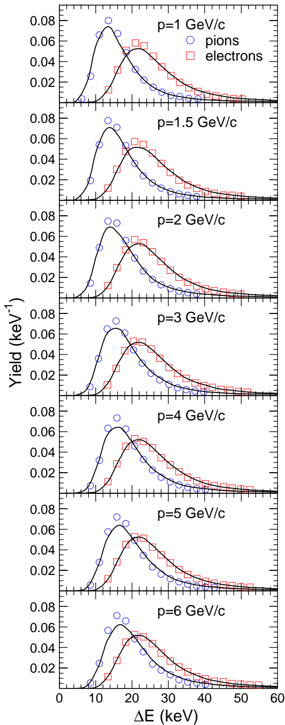
Fig. 6. The energy loss distributions of pions and electrons for momenta of 1–6 GeV/c. The symbols represent the measurements, the lines are the simulations.
