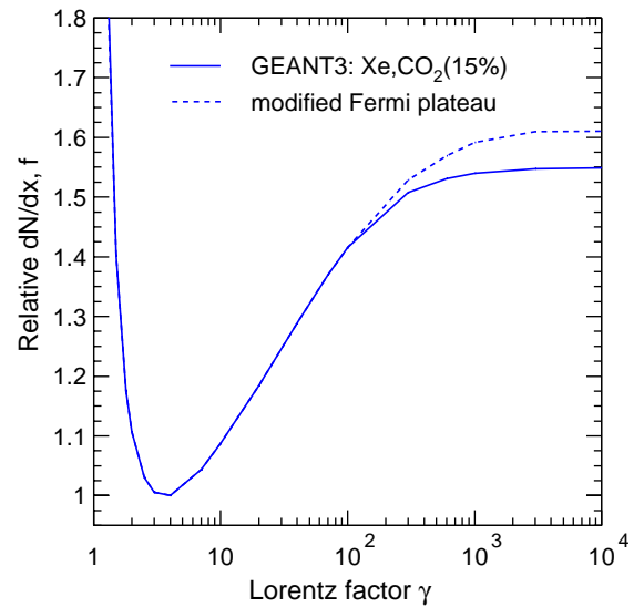
Fig. 3. The dependence of the primary number of inelastic collisions normalized to MIP ( \gamma = 4 ) on the Lorentz factor. The full line is obtained using GEANT3, the dashed line is for an increased value of the Fermi plateau that best reproduces our measurements.
