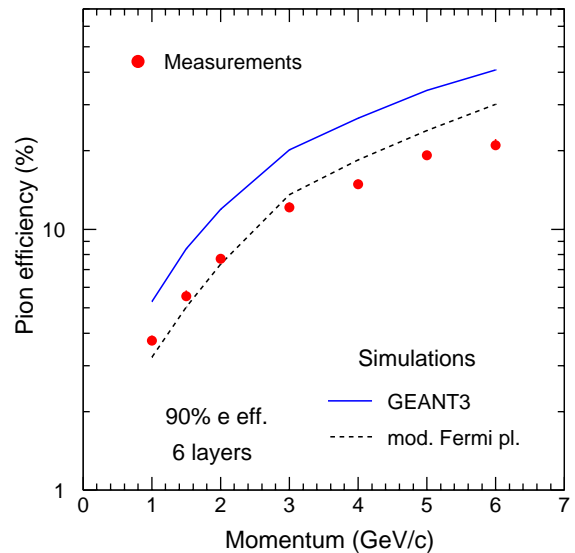
Fig. 10. The momentum dependence of the pion efficiency for 90% electron efficiency. The measurements for four layers are used to calculate the expected performance for six layers. The lines are the results of simulations.
