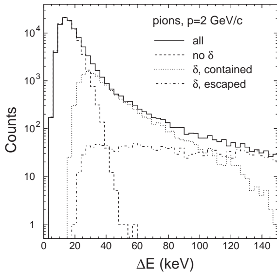
Fig. 4. Calculated integrated energy loss in our detector for 2 GeV/c pions for: (i) all tracks (full histogram), (ii) tracks which do not have any \delta -ray (dashed), (iii) tracks with \delta -rays which are contained in the detector (dotted), and (iv) tracks for which a \delta -ray has escaped the detector volume (dot-dashed).
