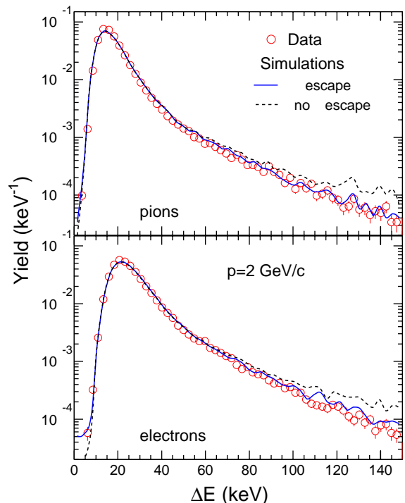
Fig. 5. Spectra of the energy loss of pions and electrons for the momentum of 2 GeV/c. The symbols represent the measurements. The lines are the simulations, with (continuous line) and without (dashed line) taking into account the finite range of \delta electrons.
