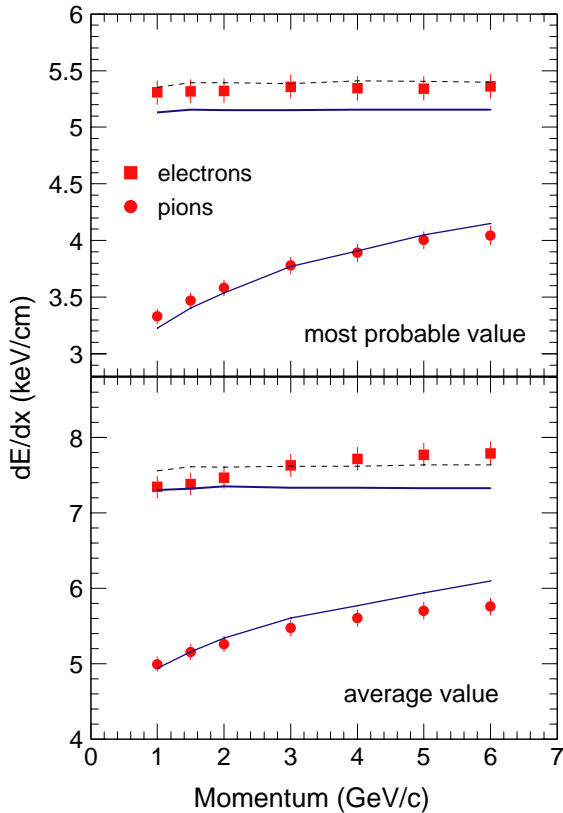
Fig. 7. Momentum dependence of the most probable and the average values of the energy loss for pions and electrons. The symbols are measurements, the lines are calculations (dashed line for the modified Fermi plateau).
