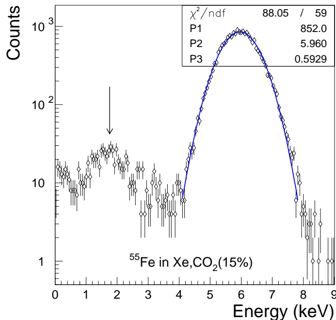
Fig. 1. ^{55}\text{Fe} spectrum in \text{Xe}, \text{CO}_2(15\%) . A Gaussian fit of the main peak of 5.96 \text{ keV} is also plotted. The arrow marks the expected position of the escape peak of Xe at 1.76 \text{ keV} .
