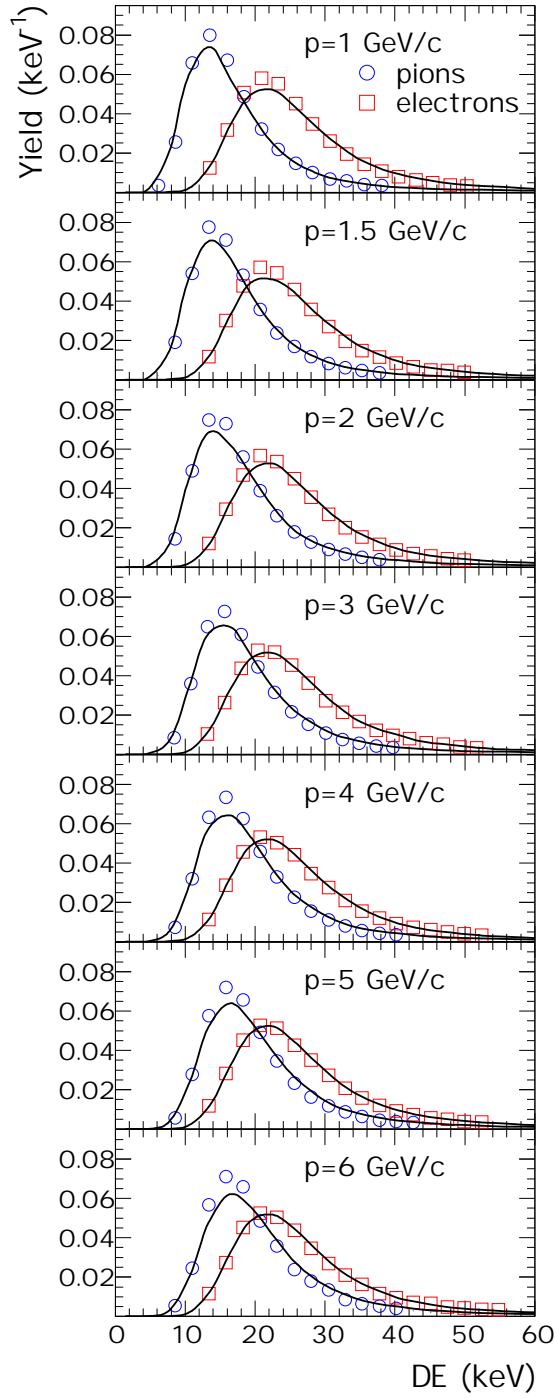
Fig. 6. The energy loss distributions of pions and electrons for momenta of 1 to 6 GeV/c. The symbols represent the measurements, the lines are the simulations.
