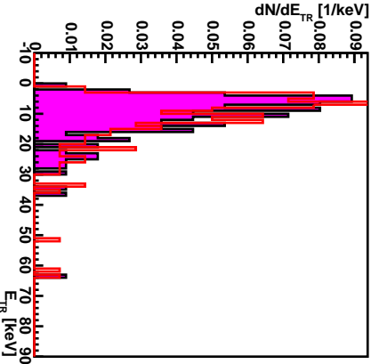
Energy of TR photons
