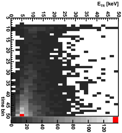
TR Absorption
